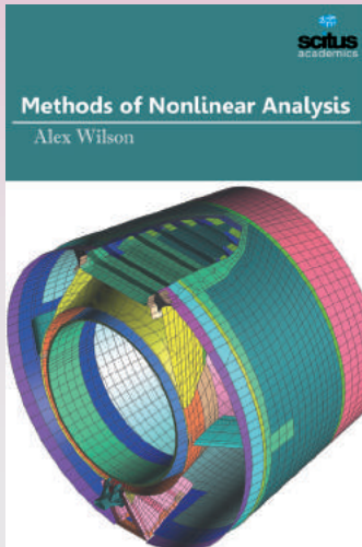
Methods of Nonlinear Analysis
