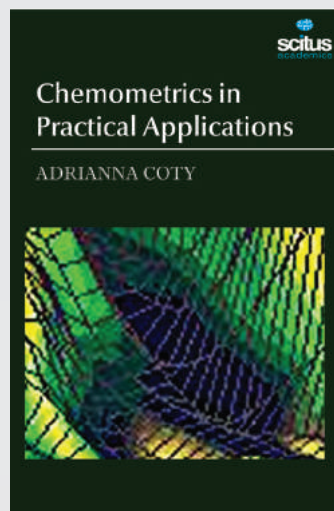
Chemometrics in Practical Applications
