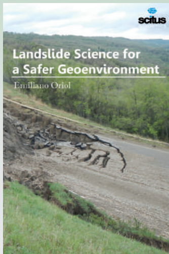
Landslide Science for a Safer Geoenvironment
