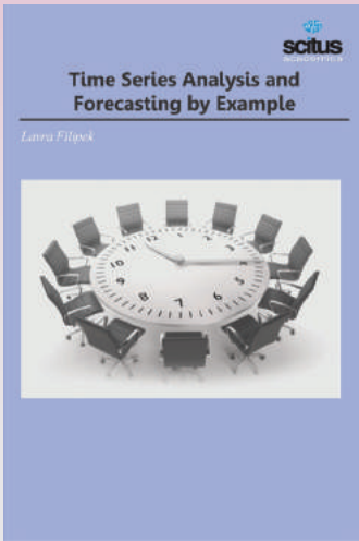
Time Series Analysis and Forecasting by Example
