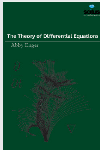
The Theory of Differential Equations
