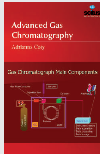
Advanced Gas Chromatography
