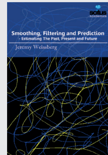
Smoothing, Filtering and Prediction - Estimating The Past, Present and Future
