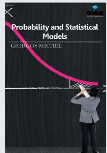
Probability and Statistical Models
