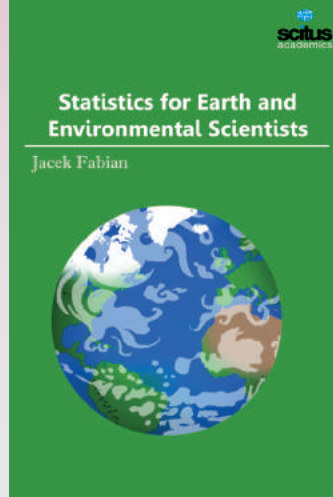
Statistics for Earth and Environmental Scientists
