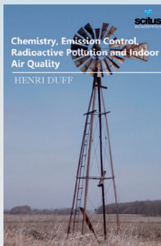
Chemistry, Emission Control, Radioactive Pollution and Indoor Air Quality
