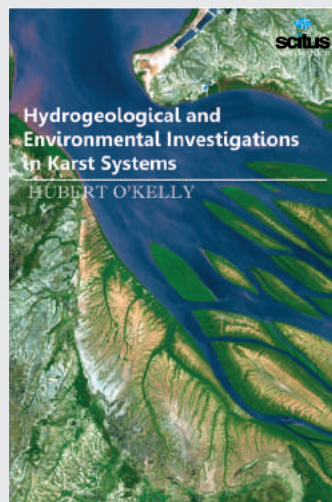
Hydrogeological and Environmental Investigations in Karst Systems
